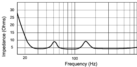
ARS-215 Impedance
