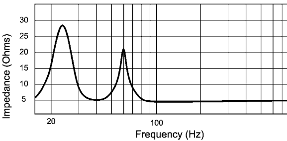
ARS-218 Impedance
